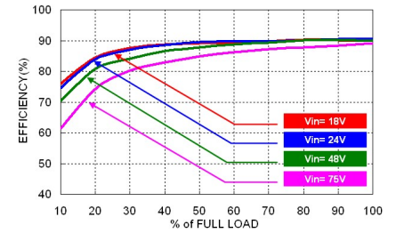
RCD20-48S05W Efficiency vs. Output Load
