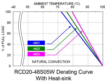
RCD20-48S05W Derating Curve
